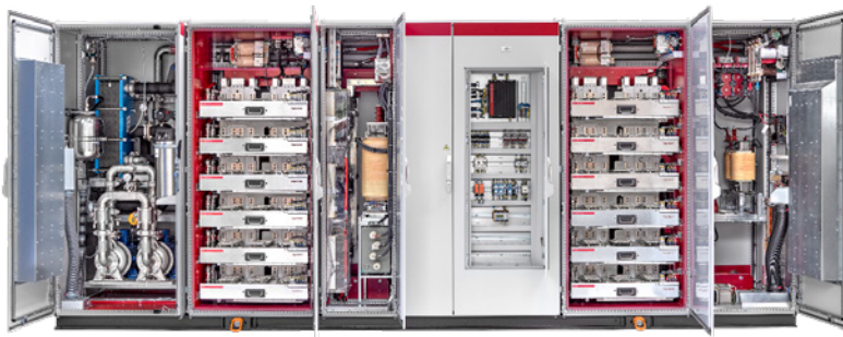
6.6 kV Medium Voltage converter solutions Power range: 10 - 137 MVA Converter: Liquid cooling Container: Ambient air cooling included
