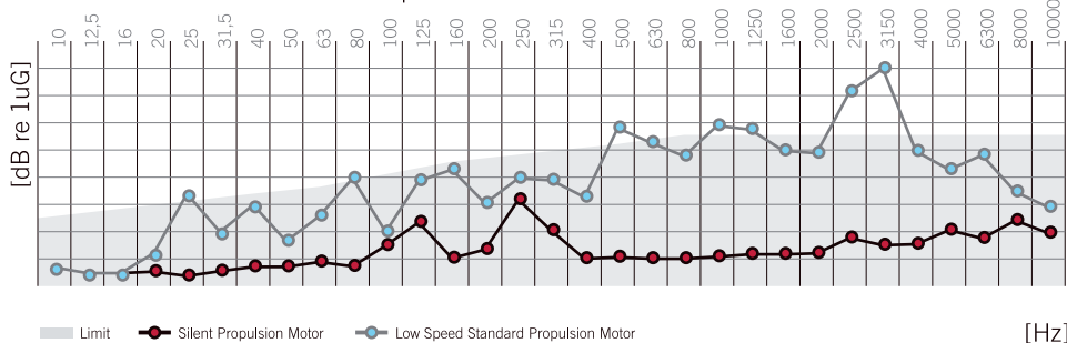
Structureborne noise Level on Propulsion Motor
