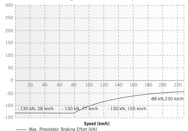
Braking Effort in fonction of speed.
