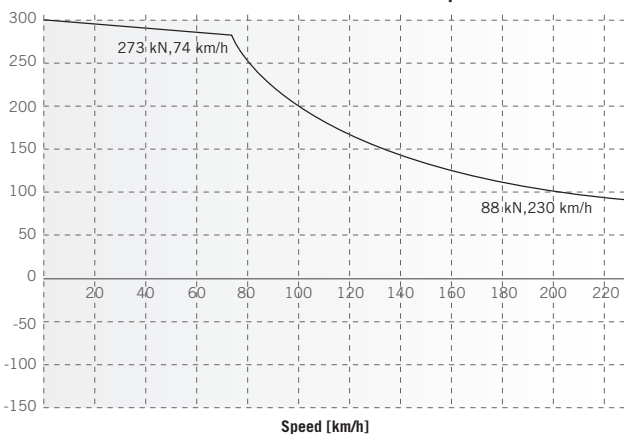
Traction Effort in fonction of speed
